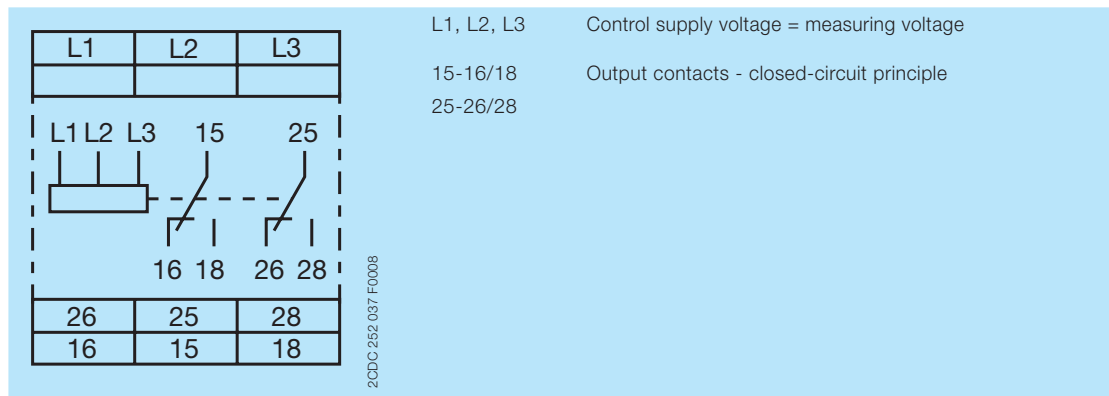
Connection diagram CM-PVS.x1
